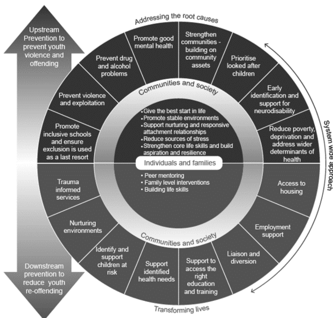
Figure 1: CAPRICORN framework
